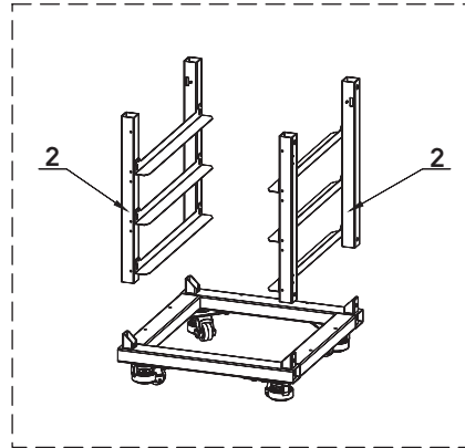
Align side racks to the bottom rack
